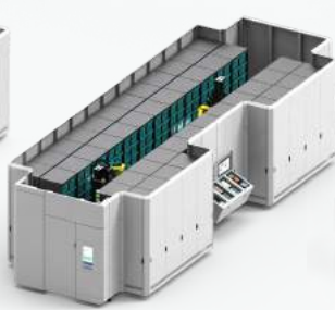
Expanded 40ft module ~43 sqm / ~430 sq. ft. (480 totes / ~1,500 SKUs)
