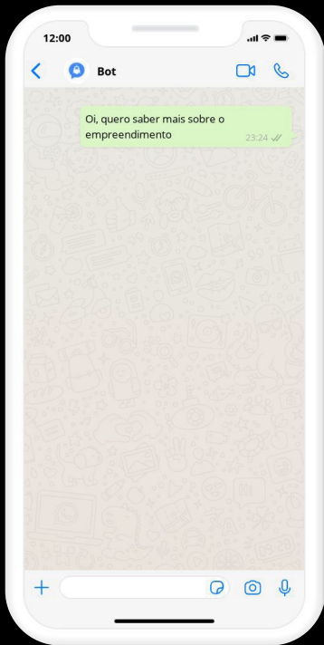
Chatbot
