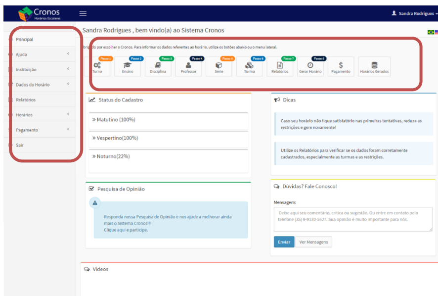
Figura 6 - Tela Principal
