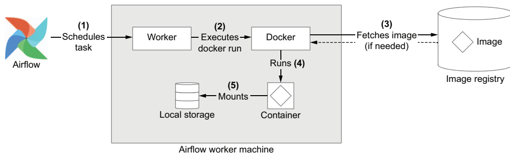
Figure 10.7 Illustration of what happens when a task is executed using the DockerOperator . The image registry stores a collection of Docker images This can be a private registry (containing our own images), or a public registry like DockerHub (which is used by default when fetching images). Images are cached locally when fetched so that you only have to do it once (barring any updates to the image).
