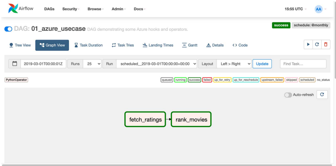
Figure 17.13 Successfully generating movie rankings using Azure Synapse in the movie ranking DAG
