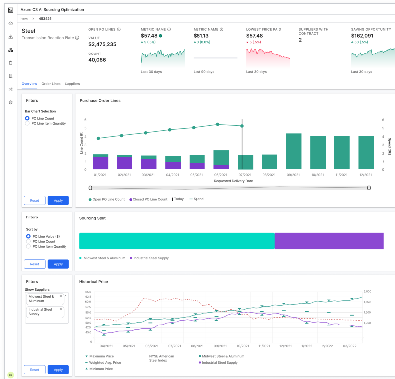
Figure 2. Azure C3 AI Sourcing Optimization enables detailed spend analysis across items and suppliers.
