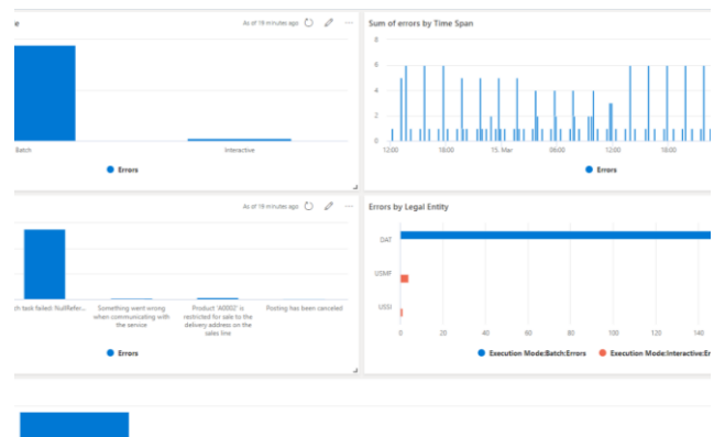
Exception view
