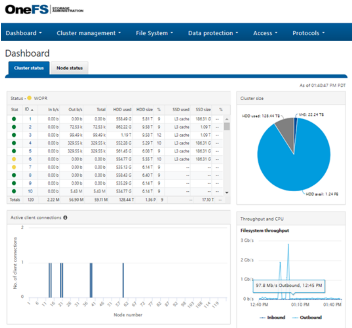
Figure 27. OneFS Web User Interface
