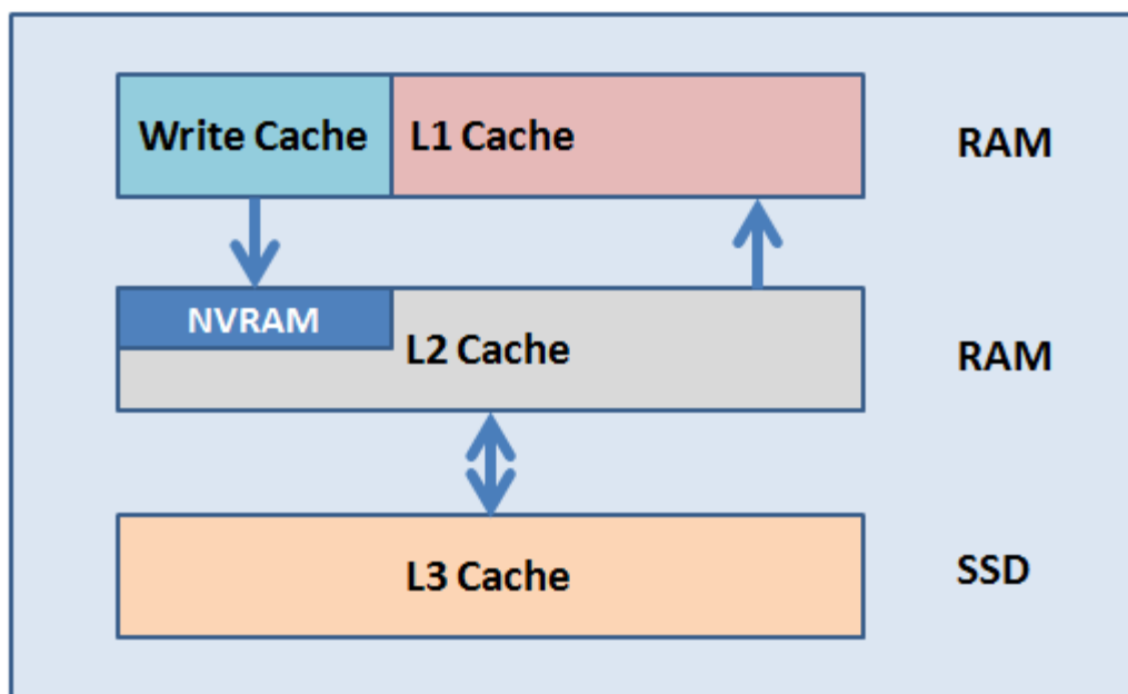
Figure 9. OneFS caching hierarchy
