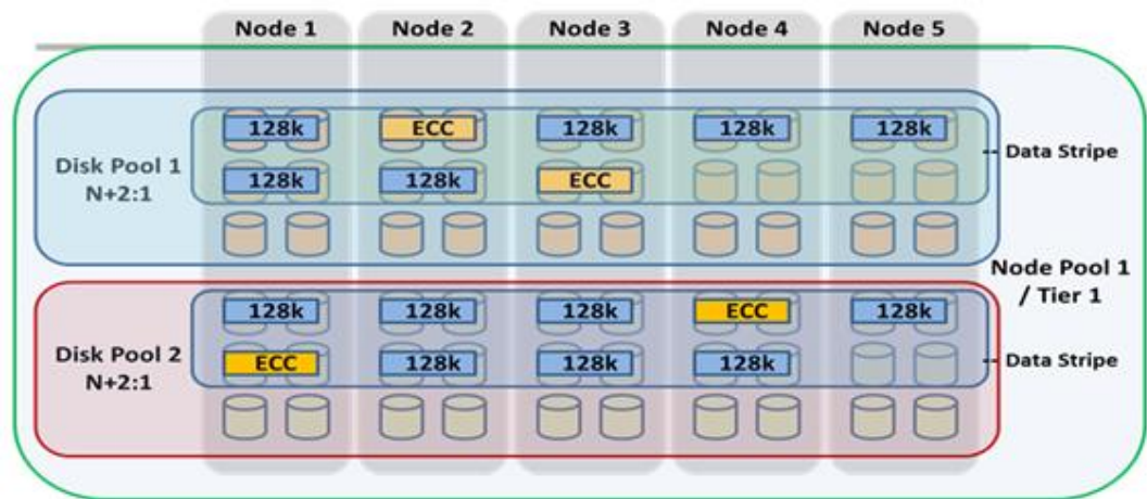
Figure 17. Automatic partitioning with SmartPools
