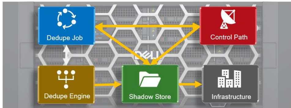
Figure 22. OneFS SmartDedupe modular architecture
