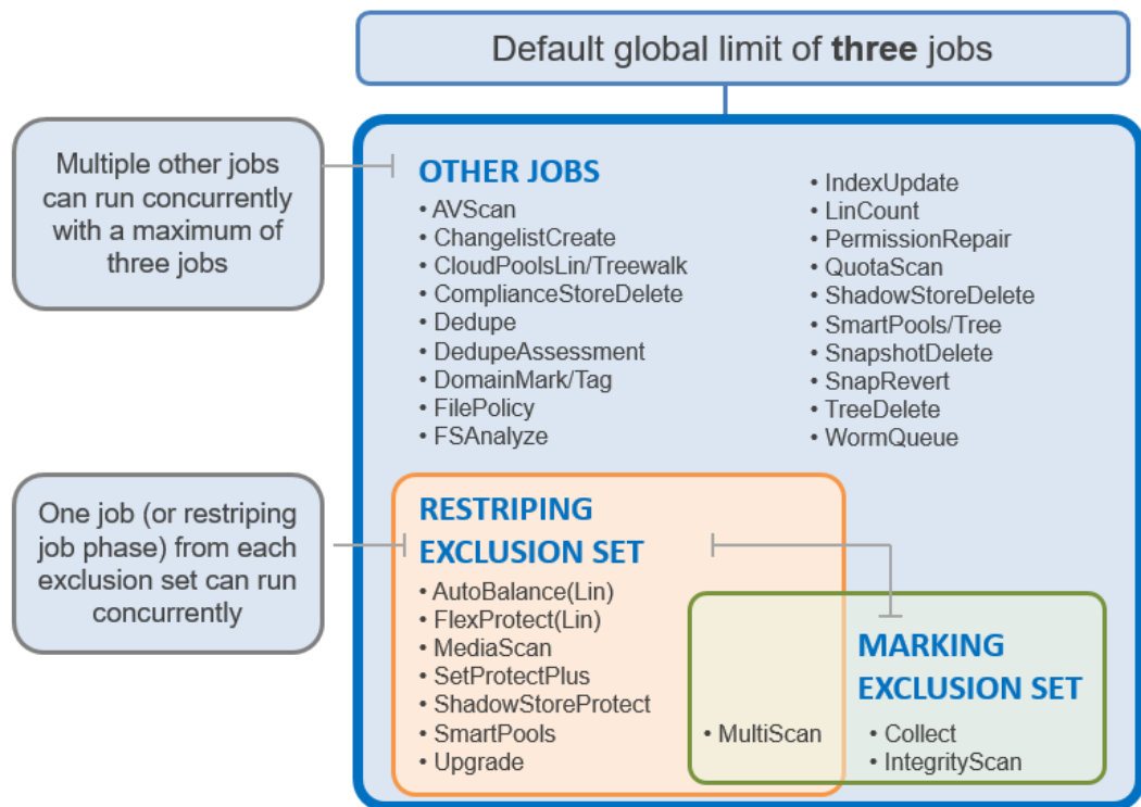
Figure 4. OneFS Job Engine Exclusion Sets
