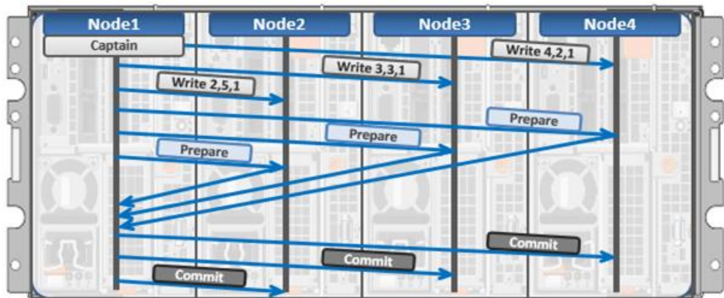
Figure 8. Distributed transactions and two-phase commit
