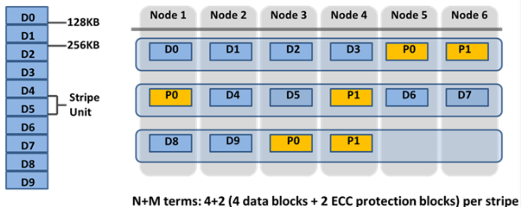
Figure 15. OneFS redundancy—N+M erasure code protection
