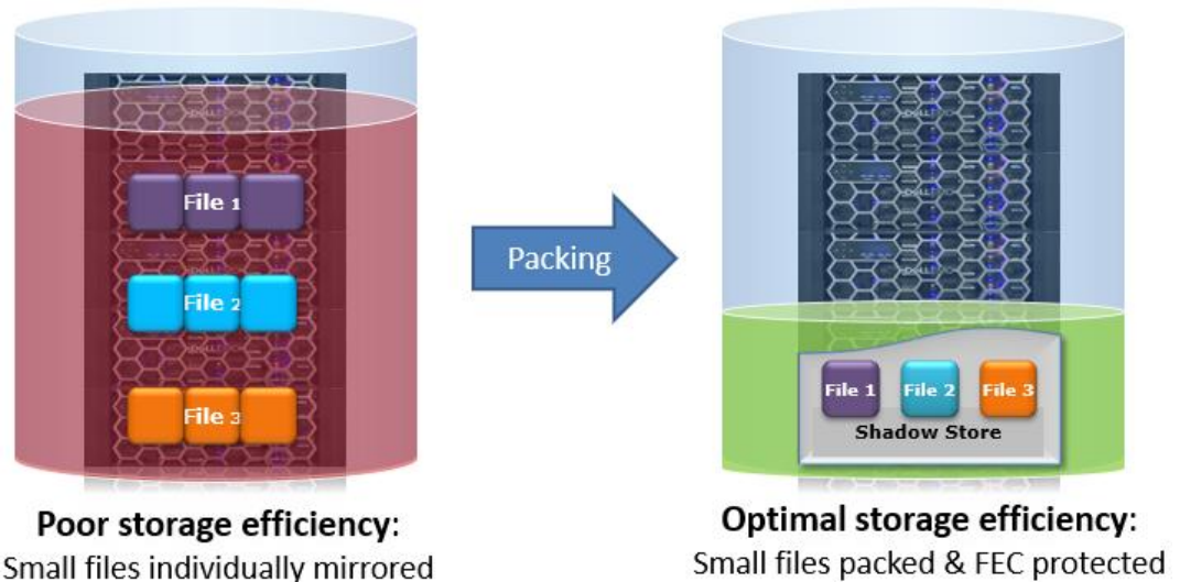
Figure 23. Small file containerization
