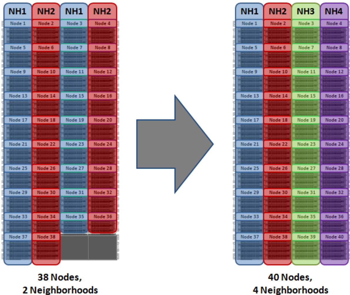
Figure 21. OneFS neighborhoods—Four neighborhood split
