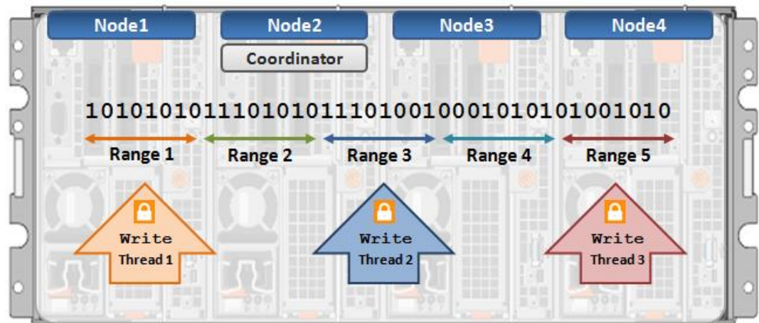
Figure 14. Multi-threaded IO writer
