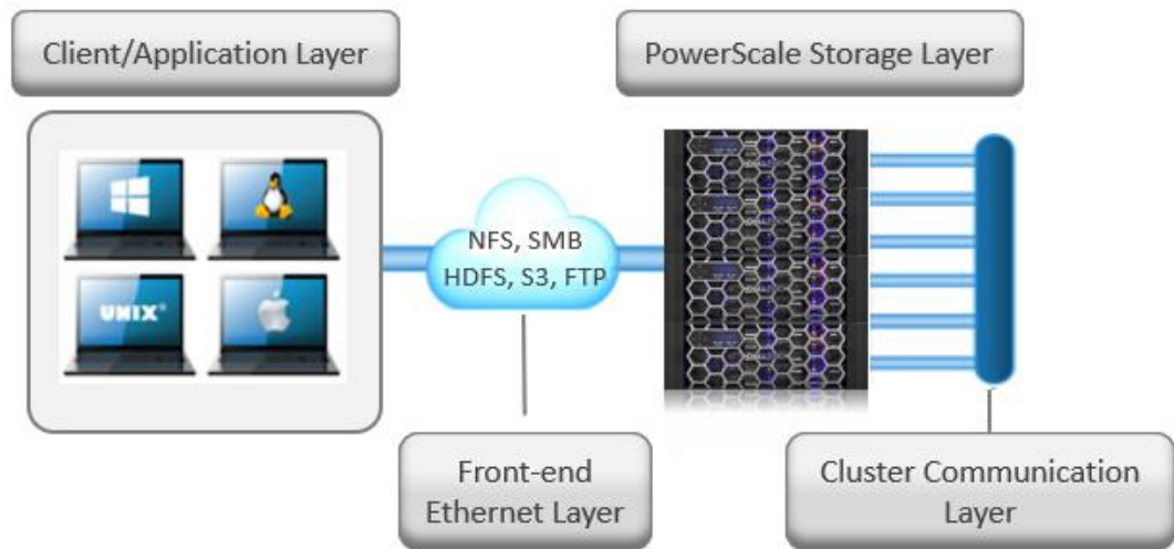
Figure 3. All components of OneFS at work
