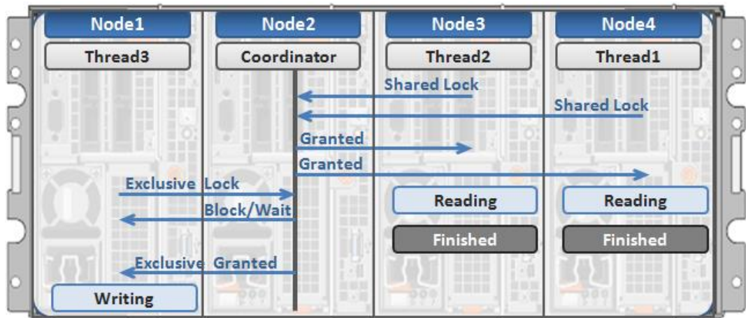
Figure 13. Distributed lock manager
