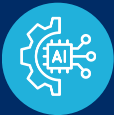
AI operations
