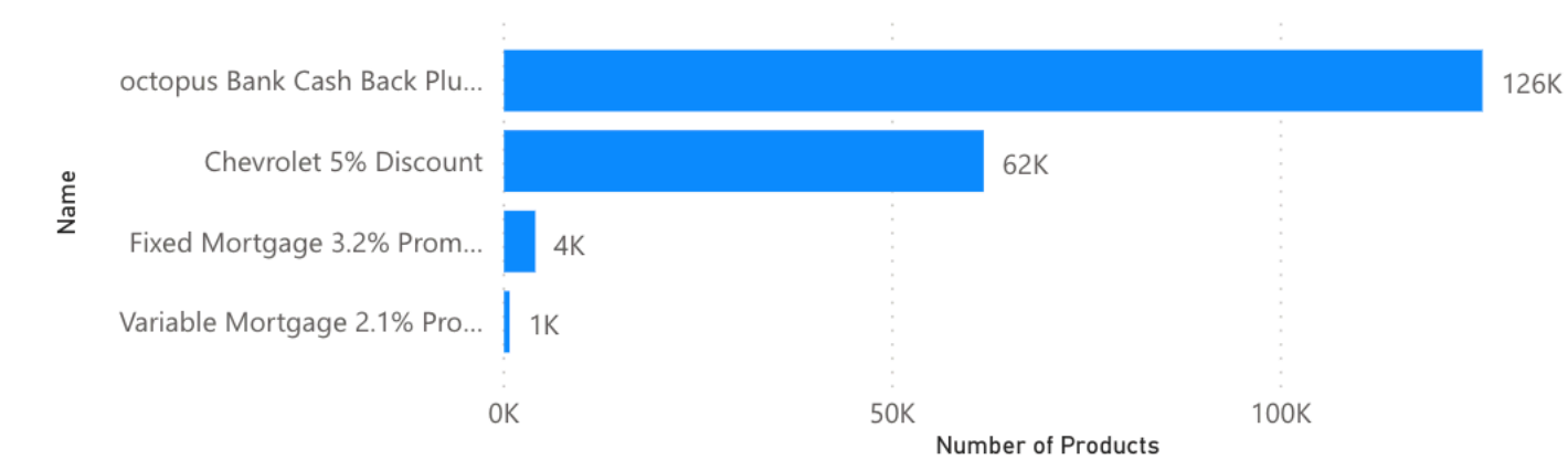
Number of Products by Name
