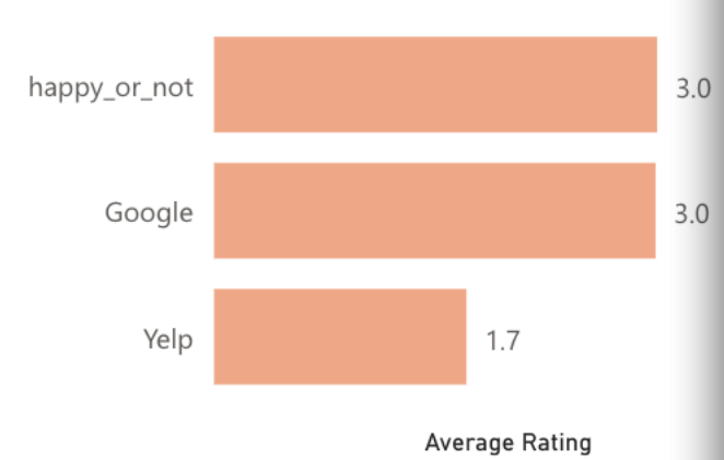
Average Rating and Average Rating All by
