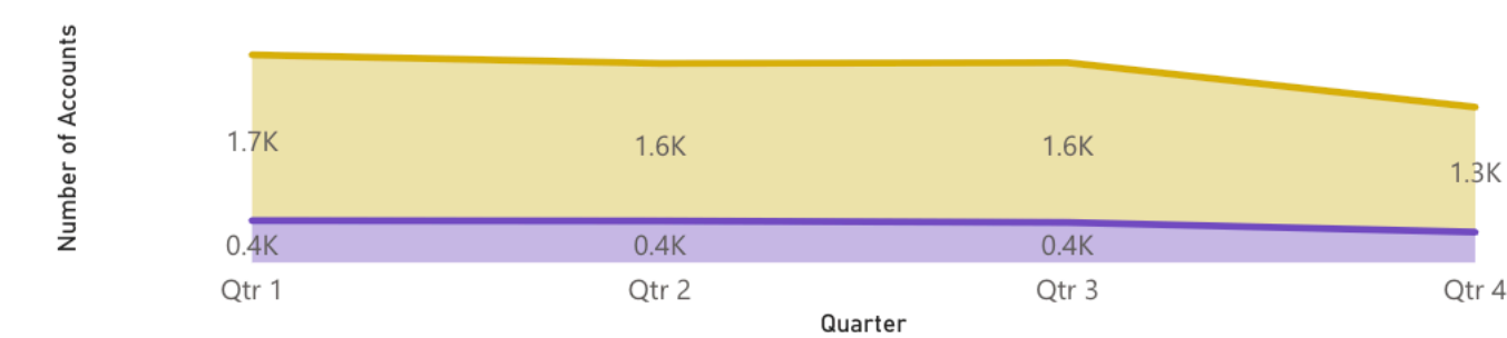
Number of Accounts by Quarter and metric
