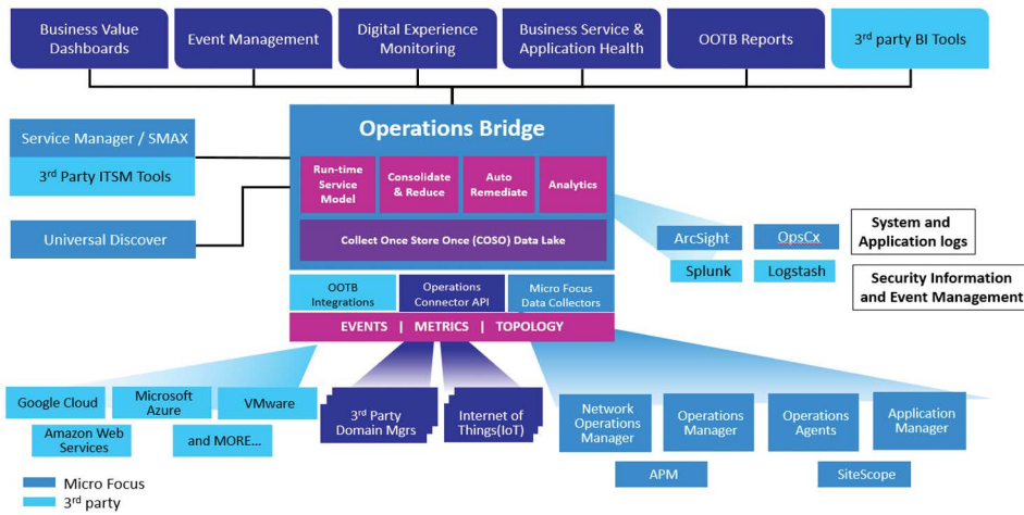
Figure 1. OpsBridge is a single consolidation console for all IT events.
