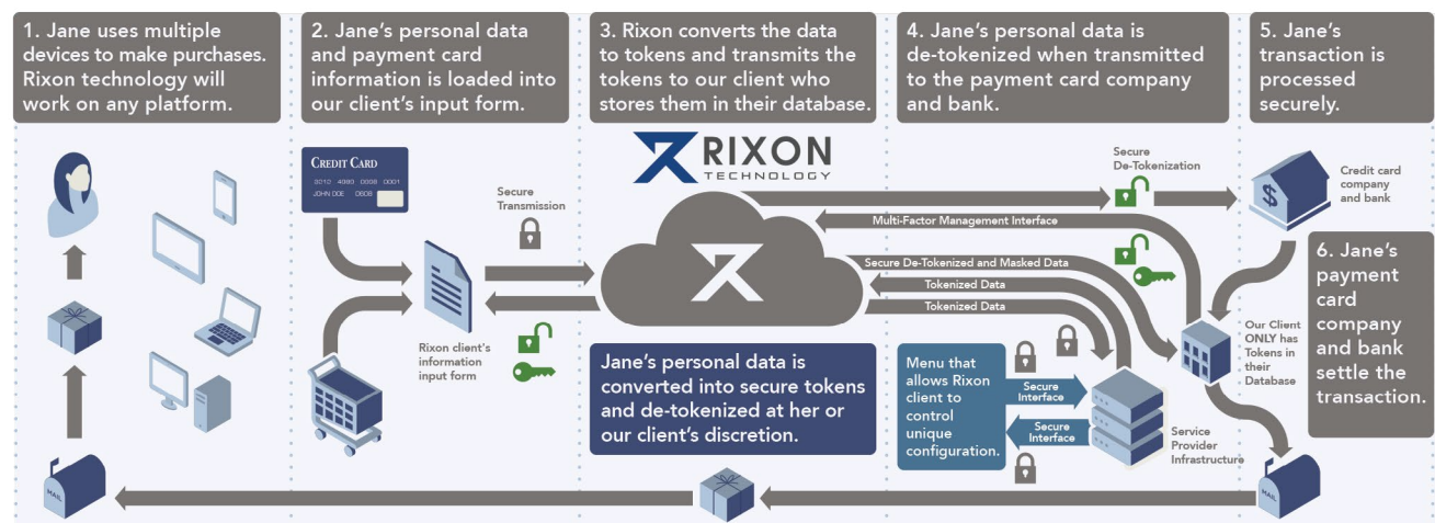
Figure 2 - Reference architecture for the vaultless tokenization process.
