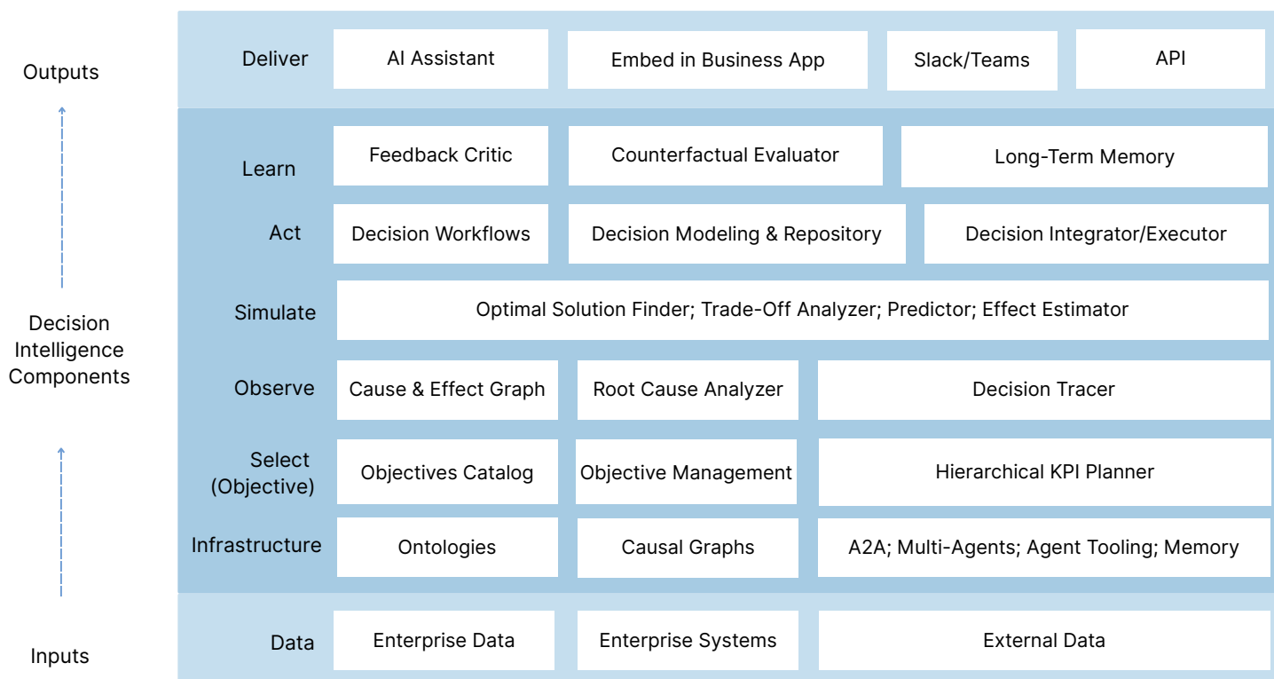
ProfitOps Decision Intelligence Stack
