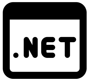
Asp.net Core
