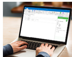
Outlook Add-on
