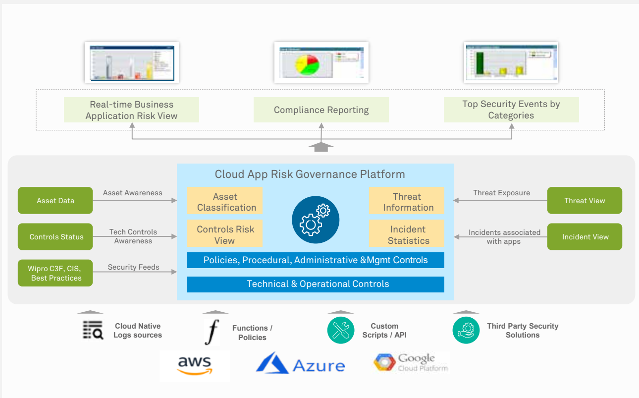
Figure 1: Cloud App Risk Governance – Continuous Controls Monitoring Framework
